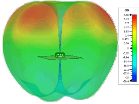
Typical 3D Pattern LTE Elements Side 800MHz
