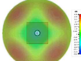
Typical 3D Pattern - LTE Elements Top 2100MHz
