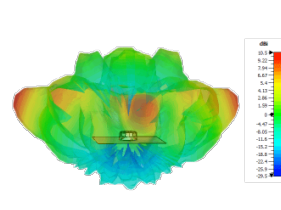
Typical 3D Pattern WiFi Elements Side 5400MHz
