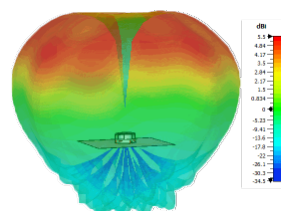
Typical 3D Pattern LTE Elements Side 2600MHz
