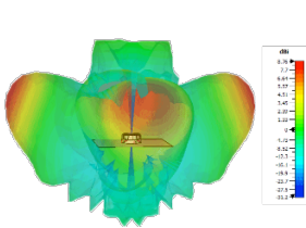
Typical 3D Pattern WiFi Elements Side 2450MHz
