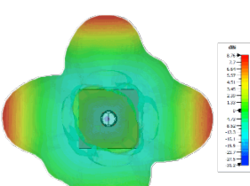
Typical 3D Pattern - WiFi Elements Top 2450MHz
