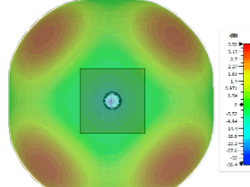
Typical 3D Pattern - LTE Elements Top 800MHz
