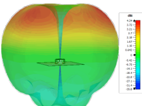
Typical 3D Pattern LTE Elements Side 2100MHz
