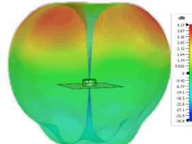
Typical 3D Pattern LTE Elements Side 1800MHz
