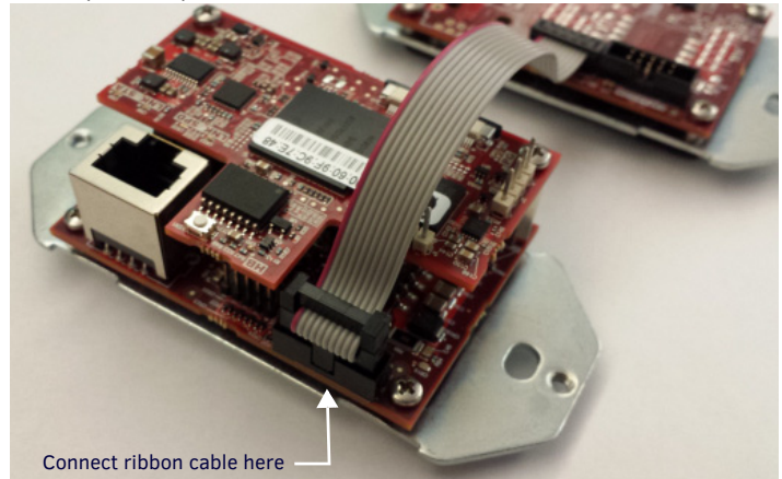
FIG. 1 DAISY-CHAIN CONNECTION BETWEEN THE MET-7E AND AN ETHERNET EXPANSION KEYPAD
