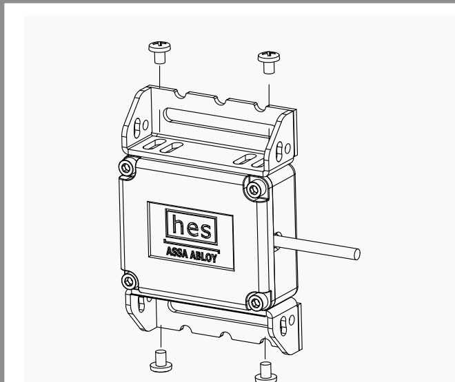
DIAGRAM 1: MOUNTING BRACKET INSTALLATION
