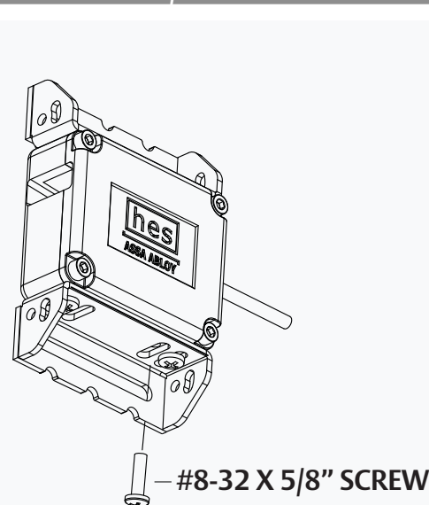
DIAGRAM 2: #8-32 X 5/8" SCREW INSTALLATION
