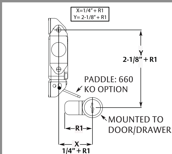
DIAGRAM 8: DIMENSIONS
