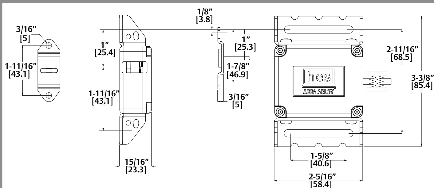
DIAGRAM 8: DIMENSIONS
