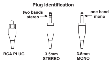
Types of plugs used with applications in this instruction manual
