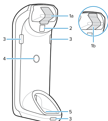
Figure 7 CR8288-SC Top Features
