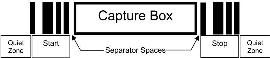
Figure 23 CapCode Structure
