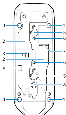
Figure 8 CR8288-SC Bottom Features
