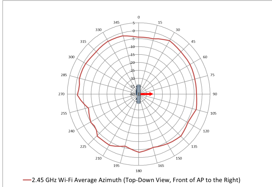
2.45 GHz Antenna Average Azimuth
