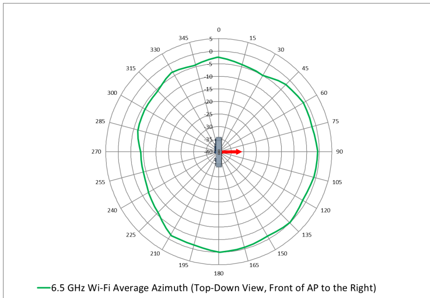
6.5 GHz Antenna Average Azimuth
