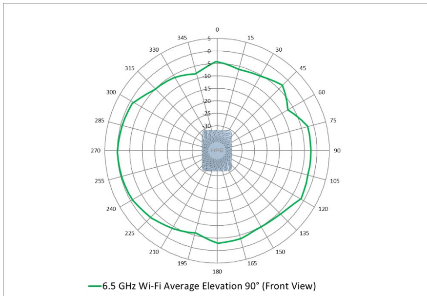
6.5 GHz Antenna Average Elevation 90 degree
