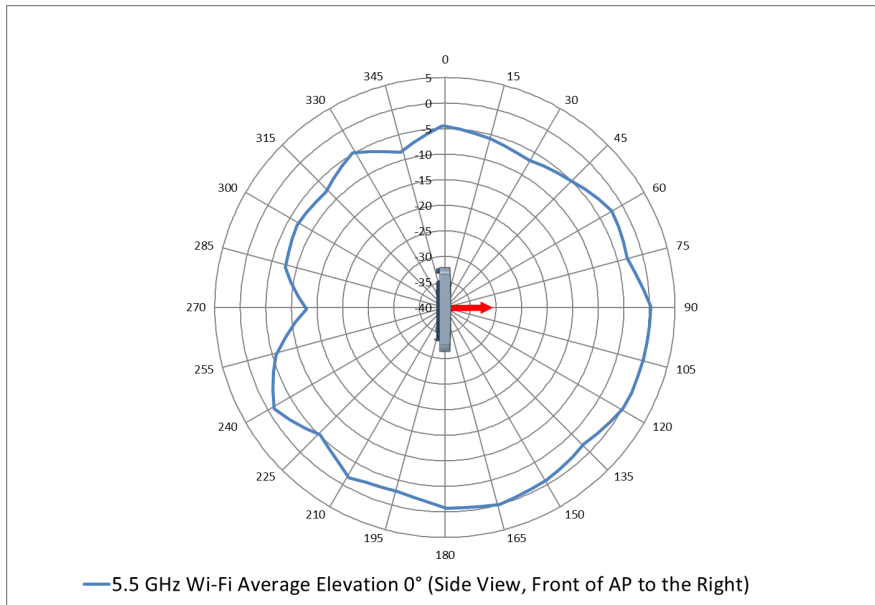
5.5 GHz Antenna Average Elevation 0 degree
