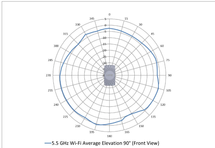
5.5 GHz Antenna Average Elevation 90 degree
