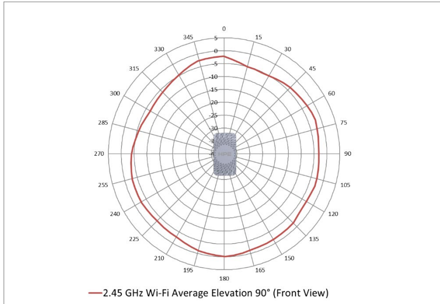
2.45 GHz Antenna Average Elevation 90 degree
