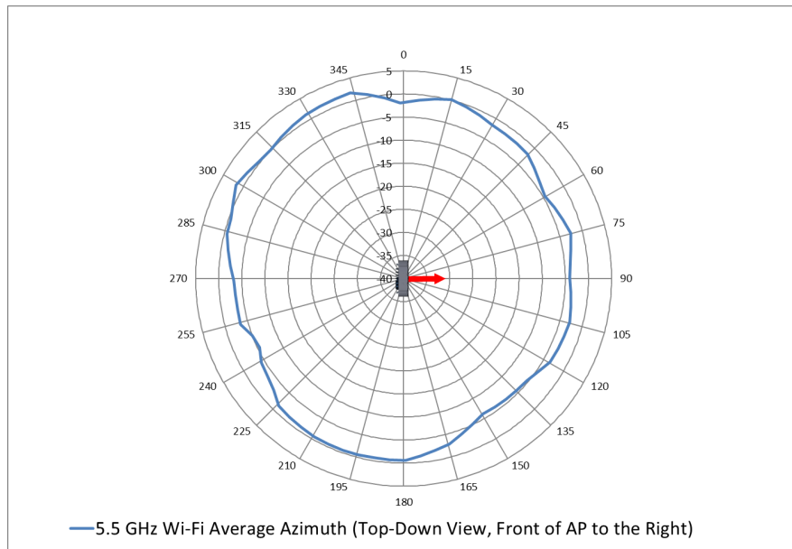
5.5 GHz Antenna Average Azimuth
