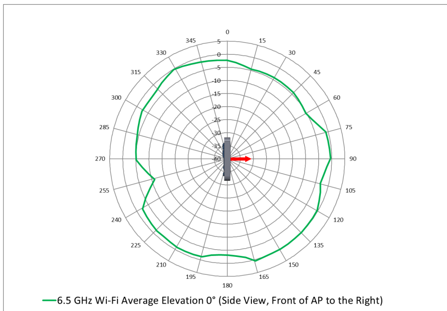
6.5 GHz Antenna Average Elevation 0 degree
