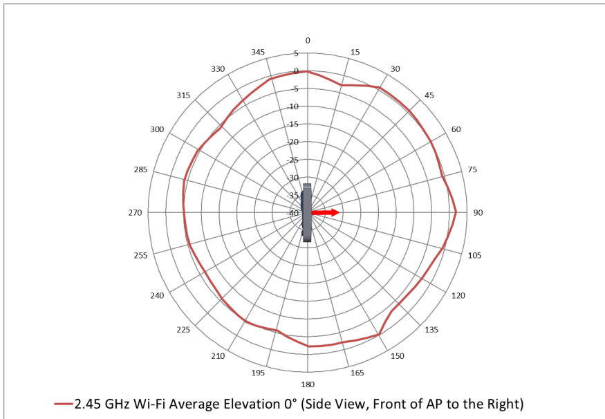
2.45 GHz Antenna Average Elevation 0 degree
