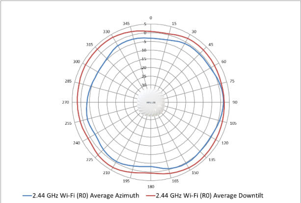
2.45 GHz Wi-Fi antenna patterns (horizontal)
