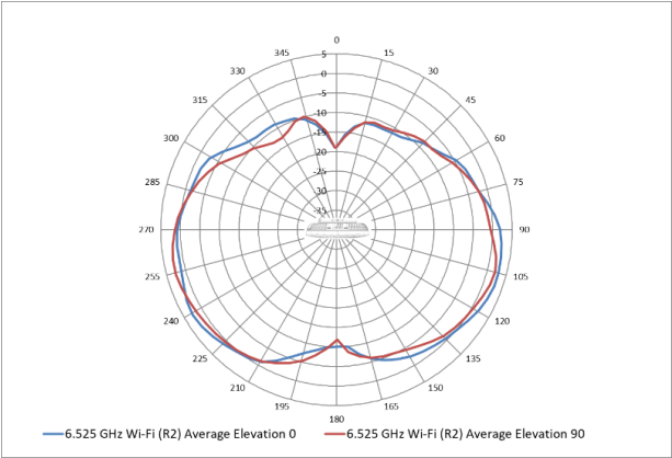
6.56 GHz Wi-Fi antennas patterns (vertical)
