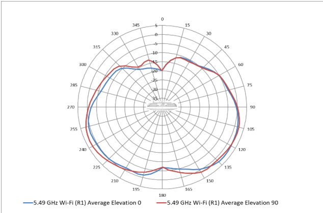
5.55 GHz Wi-Fi antenna patterns (vertical)
