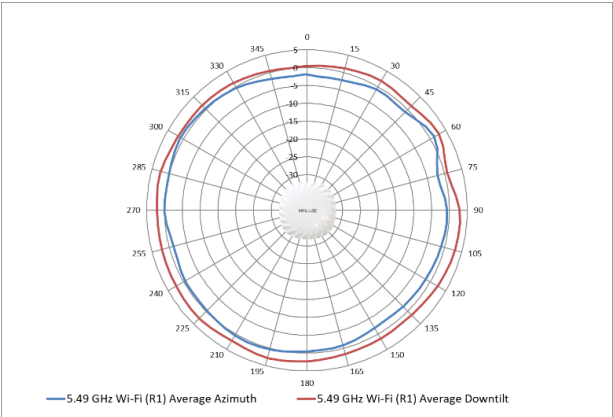
5.55 GHz Wi-Fi antenna patterns (horizontal)
