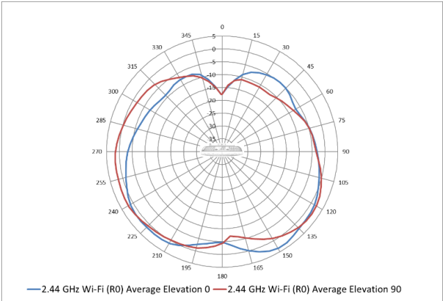
2.45 GHz Wi-Fi antennas patterns (vertical)
