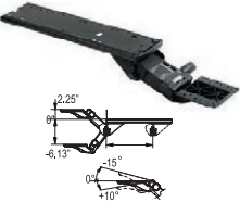
KSM02-21 Lift-N-Lock Keyboard Support Mechanism 9w x 23.8d x 9.7h $215
