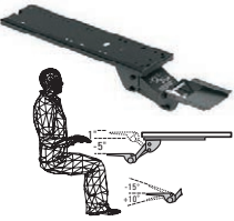
KSM01-21 Soft Touch Keyboard Support Mechanism 9w x 23.8d x 4.3h $165
