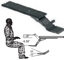
KSFK-21 Slim Fit Keyboard Support Mechanism 7.5w x 17.5d x 4.75h $215
