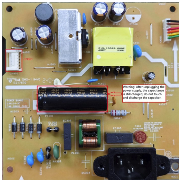
CN801 Wistron P/N: 021.61323.0106
