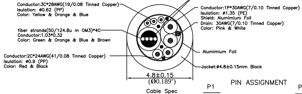
Cable TABLE:
