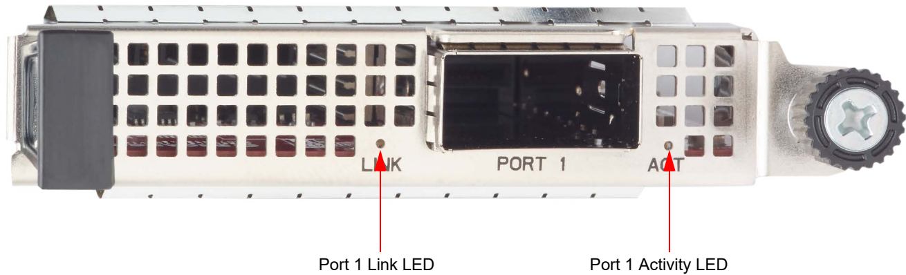
Figure 3: Activity and Link LED Locations
