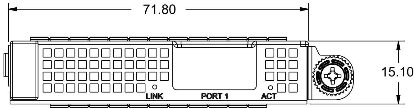
Figure 4: Physical Dimensions (in millimeters)
