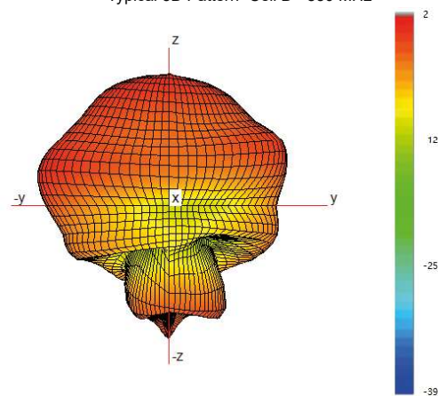
Typical 3D Pattern- Cell D - 850 MHz
