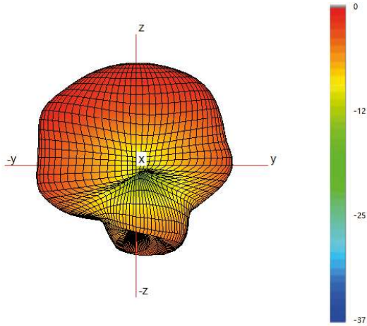
Typical 3D Pattern- Cell D - 750 MHz
