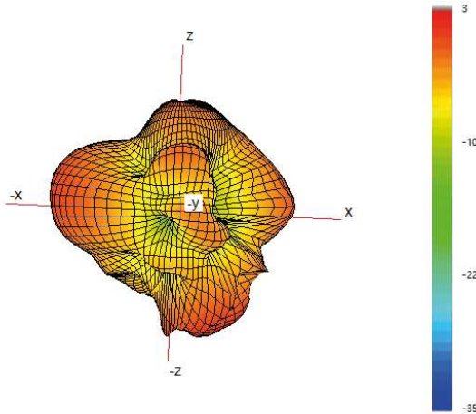
Typical 3D Pattern- Cell A - 1475 MHz
