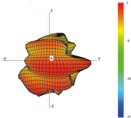
Typical 3D Pattern- Cell B - 1475 MHz
