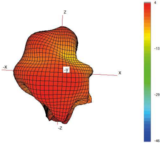
Typical 3D Pattern- Cell A - 2650 MHz
