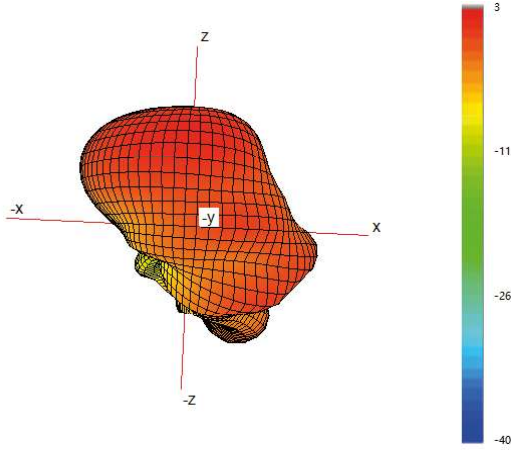
Typical 3D Pattern- Cell A - 850 MHz
