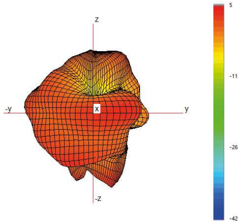
Typical 3D Pattern- Cell B - 2650 MHz
