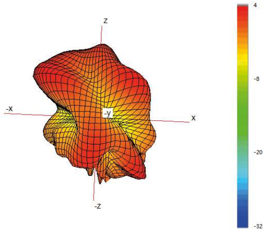
Typical 3D Pattern- Cell A - 2350 MHz
