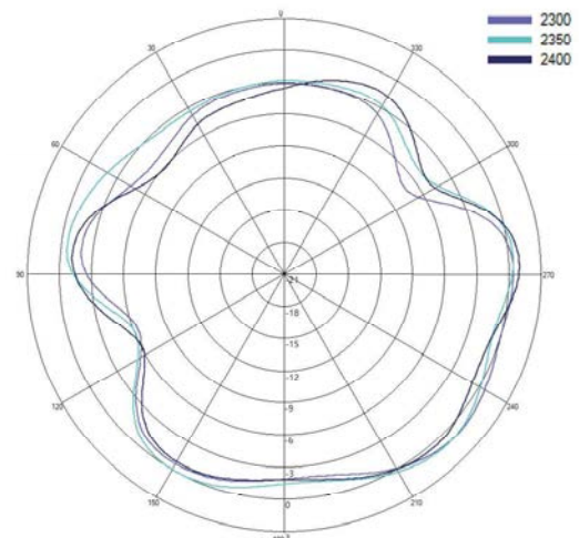
Typical H Plane- Cell D - Patterns- 2300-2400 MHz
