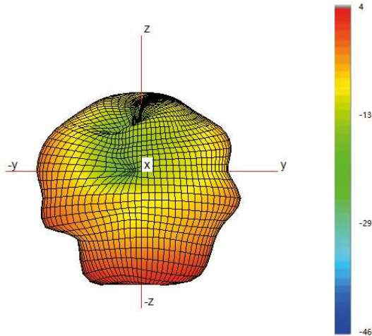
Typical 3D Pattern- Cell B - 850 MHz
