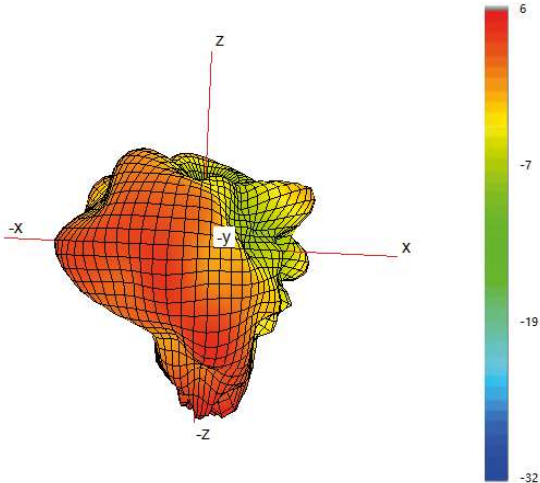
Typical 3D Pattern- Cell A - 3600 MHz
