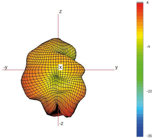
Typical 3D Pattern- Cell C - 1800 MHz
