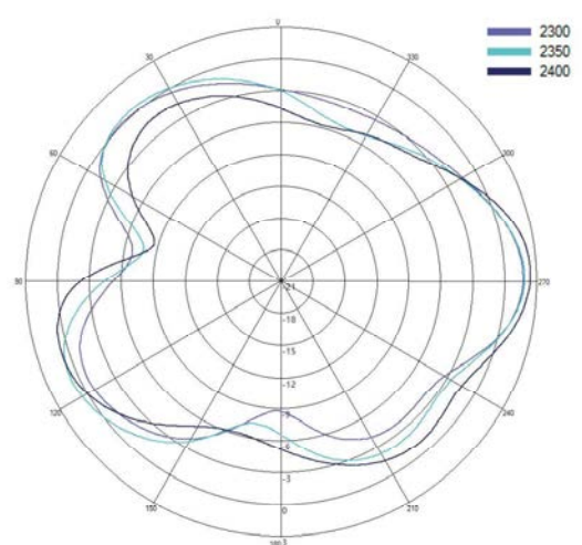
Typical H Plane- Cell C - Patterns- 2300-2400 MHz
