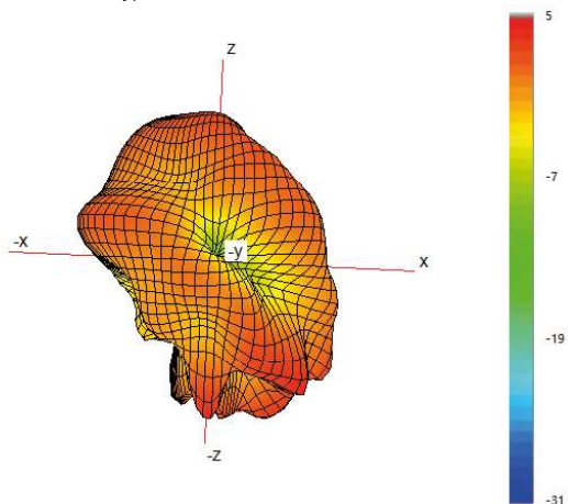
Typical 3D Pattern- Cell A - 2150 MHz
