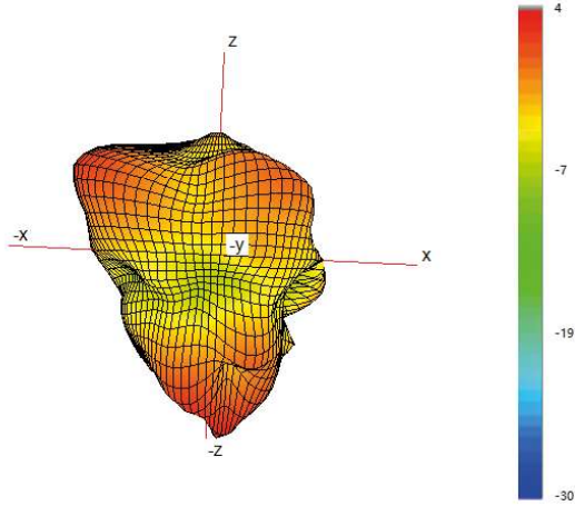
Typical 3D Pattern- Cell A - 1800 MHz
