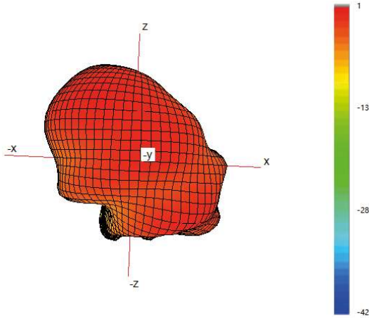
Typical 3D Pattern- Cell A - 750 MHz
