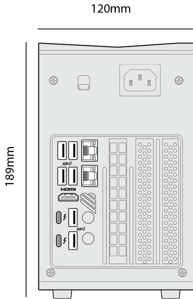
Figure 15. Back Side
