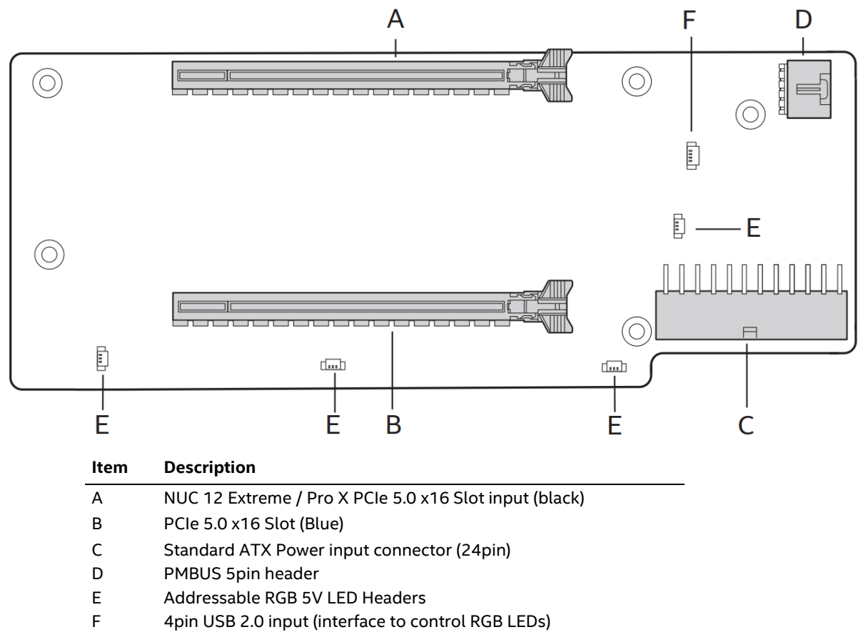
Figure 9. BBMC1B2 Baseboard Connectors
