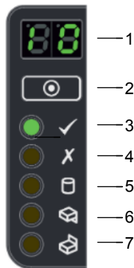
Figure 2-14 Control panel
