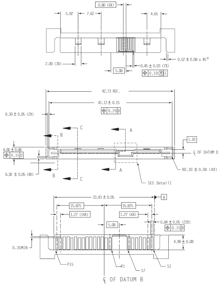
Figure 12 SAS device plug dimensions
