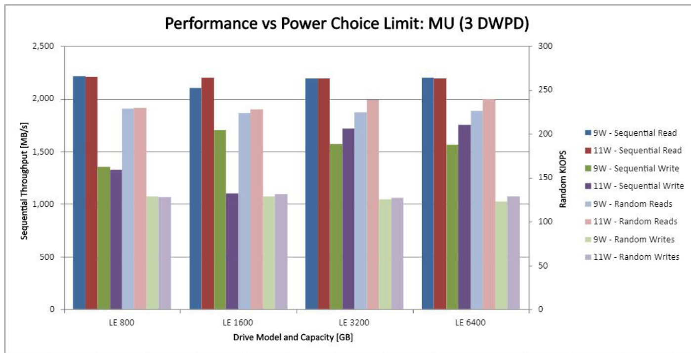
Figure 2 Mixed Use Models: Performance vs Power Limit Setting chart
