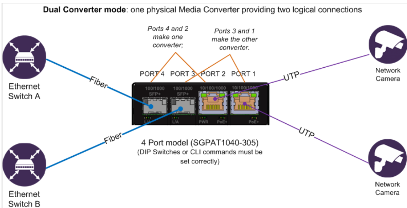
4-Port Dual-Converter Mode Example
