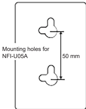
Mounting Holes for Drawing of NFI-U05A
