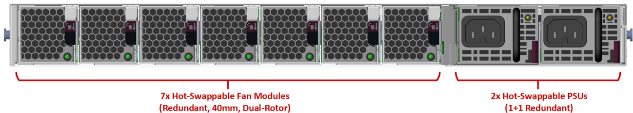
FIGURE 3. 9200TXE rear panel
