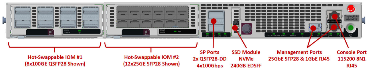
FIGURE 2. 9200TXE front panel
