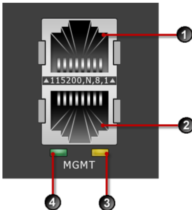
FIGURE 4. Console and management ports
