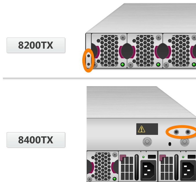
FIGURE 11. Ground screw location for TX devices
