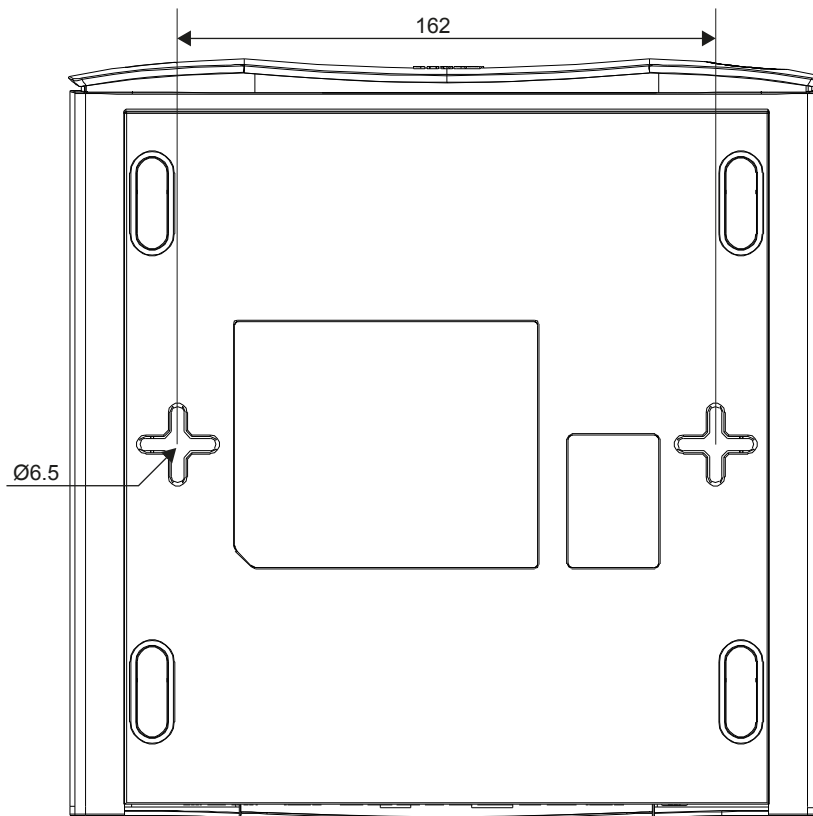
Image 3–1 Mounting holes
