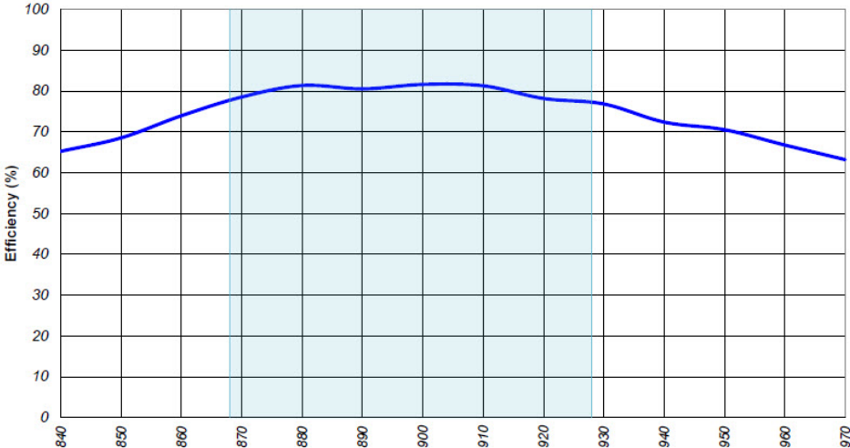
Figure 4: Efficiency Vs Frequency
