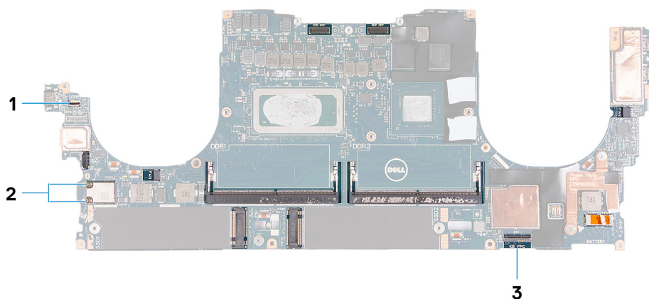
Figure 1. System-board connectors
