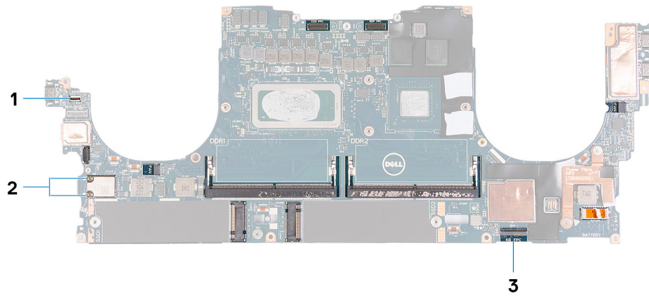
Figure 2. System-board connectors
