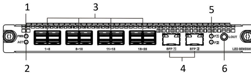
Figure 1-13 LED Sending Card
