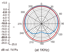
Polar Pattern
