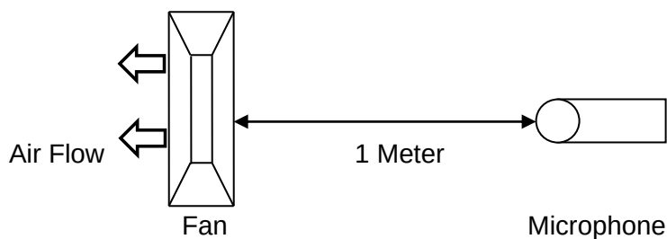
Figure A – Noise Level is measure at rated voltage in anechoic chamber in free air as above.
