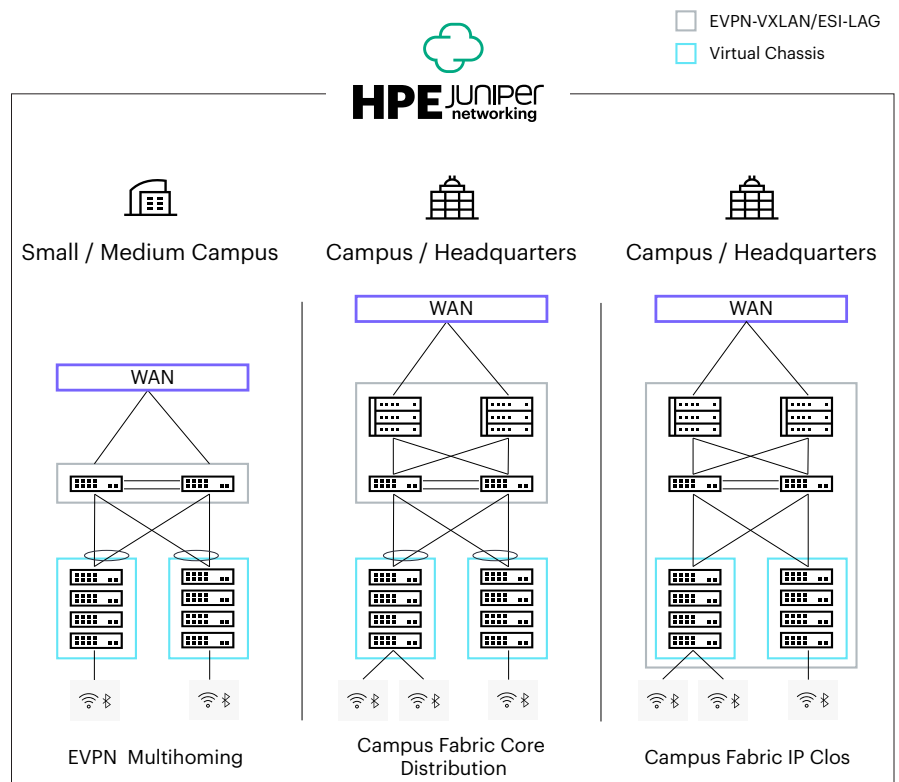
Figure 4. Campus fabrics architectures showing EX4650 in the distribution
