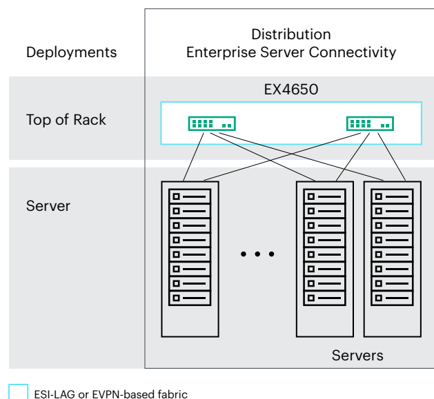
Figure 6. EX4650 for enterprise on-premises server connectivity
