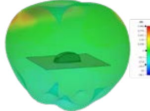
3D Plot Element 4 Side (750 MHz)
