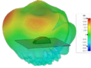
3D Plot Element 2 Side (2000 MHz)
