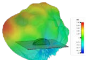
3D Plot Element 2 Side (3600 MHz)
