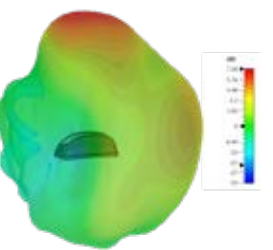
3D Plot Element 4 Side (2600 MHz)
