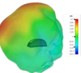
3D Plot Element 2 Side (2600 MHz)
