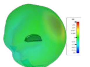
3D Plot Element 3 Side (5400 MHz)
