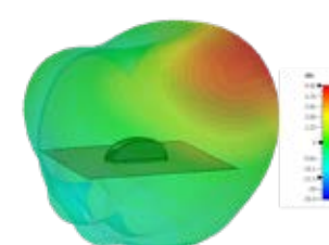
3D Plot Element 4 Side (1800 MHz)
