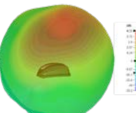
3D Plot Element 4 Side (2600 MHz)
