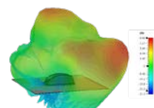
3D Plot Element 4 Side (3600 MHz)
