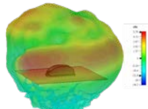
3D Plot Element 4 Side (2600 MHz)
