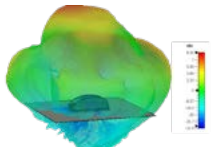
3D Plot Element 3 Side (3600 MHz)
