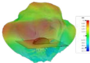
3D Plot Element 1 Side (3600 MHz)
