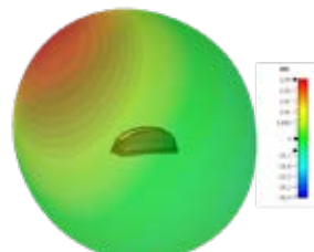
3D Plot Element 1 Side (1800 MHz)
