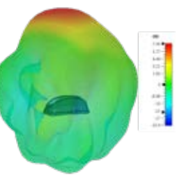
3D Plot Element 3 Side (2600 MHz)
