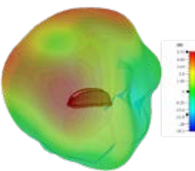
3D Plot Element 1 Side (2600 MHz)
