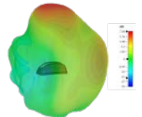
3D Plot Element 4 Side (2600 MHz)
