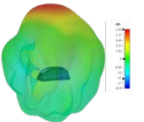
3D Plot Element 3 Side (2600 MHz)
