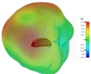
3D Plot Element 1 Side (2600 MHz)
