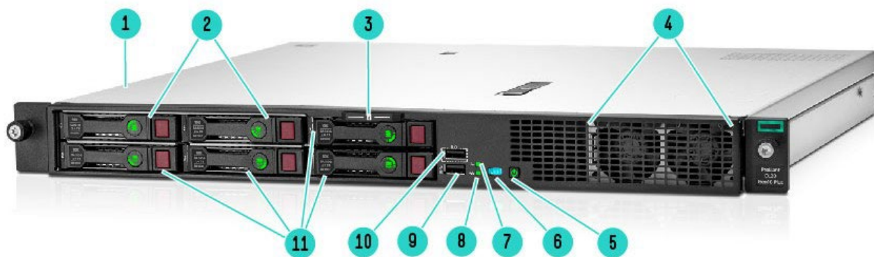
4 (+2) SFF Front View Gen10 Plus
