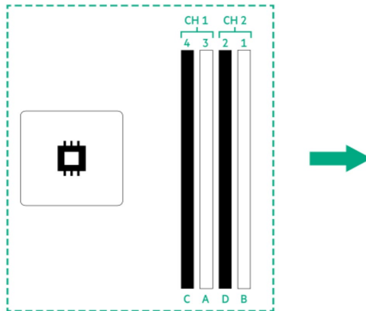
DIMM slot and configuration diagram
