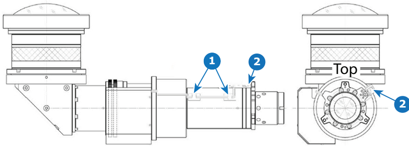
Image 4-6 90° rotated position
