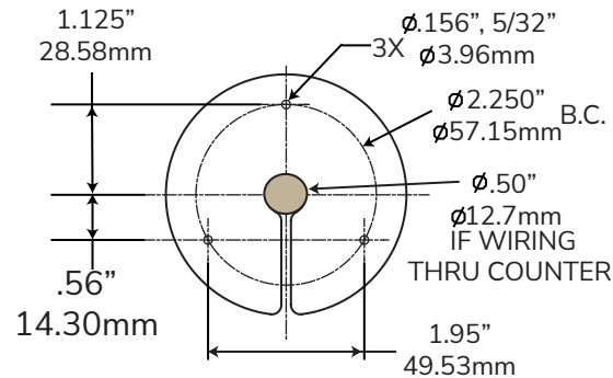
COUNTER MOUNTING
