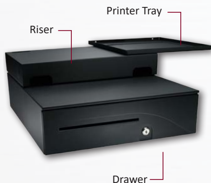
POS-Integrator™ System 16195
