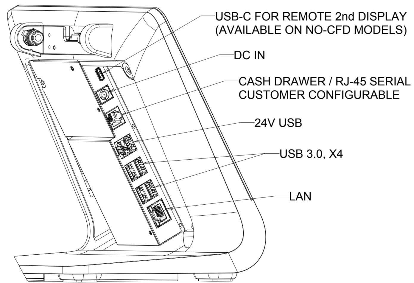
I/O DEFINITION (CABLE COVER DOOR REMOVED)
