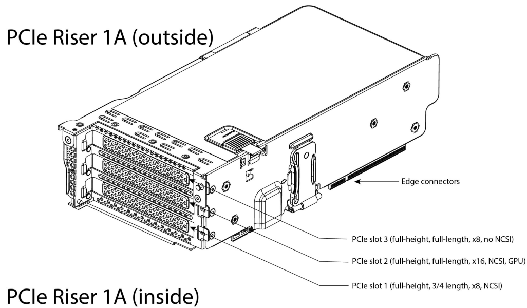
Figure 20 Riser Card 1A
