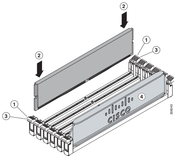
Figure 26 Replacing Memory
