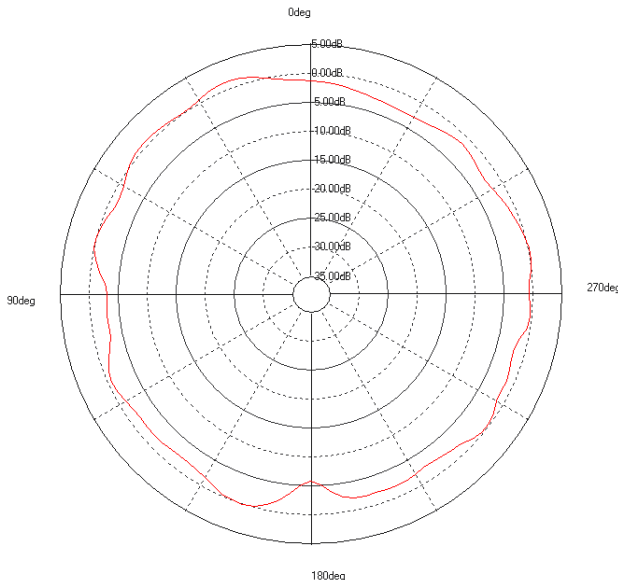
Horizontal Polarity Elevation Pattern 5150 – 5875 MHz:
