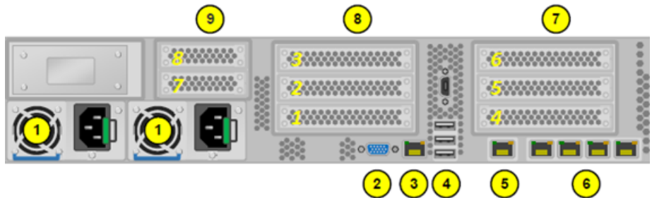
Figure 1-2 Veritas 5350 Appliance rear panel overview
