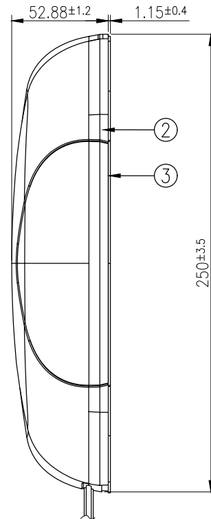
Side View
