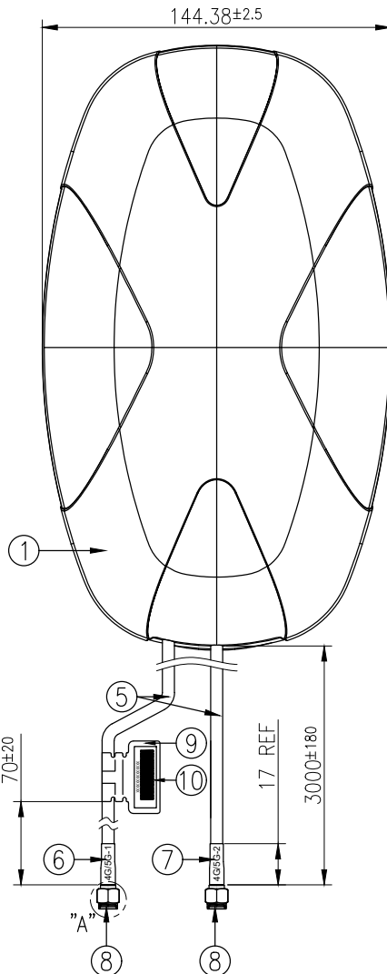
Bottom View
