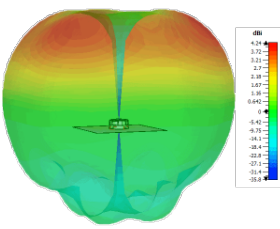
Typical 3D Pattern LTE Elements Side 2100MHz
