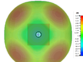
Typical 3D Pattern LTE Elements Top 1800MHz
