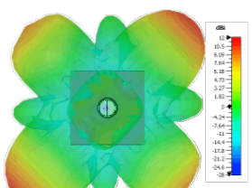
Typical 3D Pattern - LTE Elements Top 3600MHz
