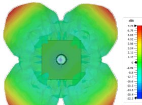
Typical 3D Pattern LTE Elements Top 2600MHz
