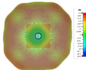
Typical 3D Pattern LTE Elements Top 2600MHz
