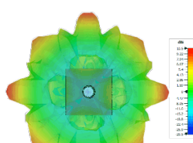
Typical 3D Pattern WiFi Elements Top 5400MHz
