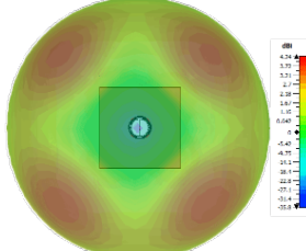
Typical 3D Pattern - LTE Elements Top 2100MHz
