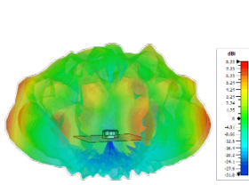
Typical 3D Pattern LTE Elements Side 5400MHz
