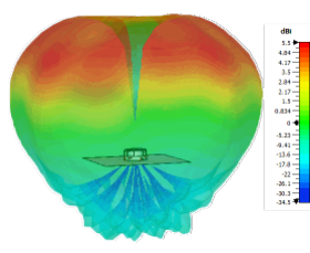
Typical 3D Pattern LTE Elements Side 2600MHz
