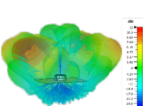
Typical 3D Pattern LTE Elements Side 3600MHz
