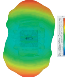
3D Gain Plot Top (3600MHz)
