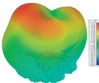
3D Gain Plot Top (5.4GHz)
