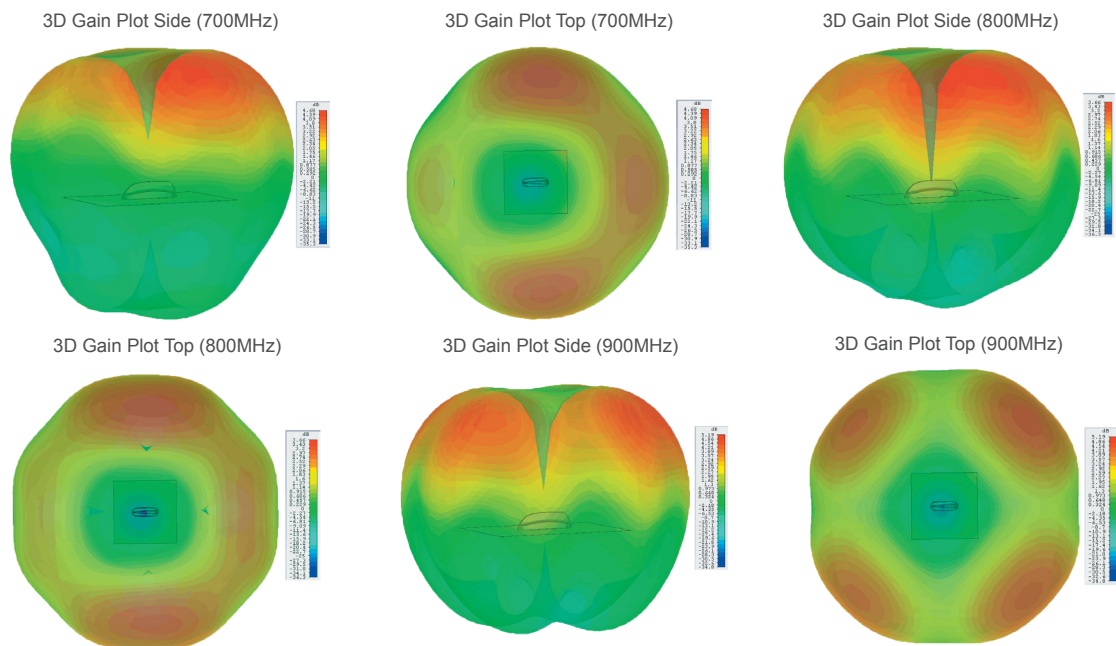
3D Radiation Patterns - Cell / LTE Elements 2&3
