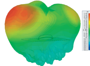
3D Gain Plot Top (2600MHz)
