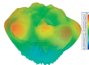
3D Gain Plot Side (5.4GHz)
