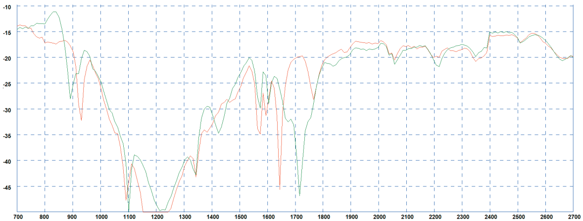
Isolation Typical Isolation - Cellular Elements 2&3*
