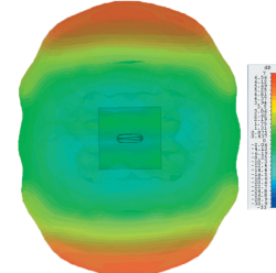
3D Gain Plot Top (2600MHz)
