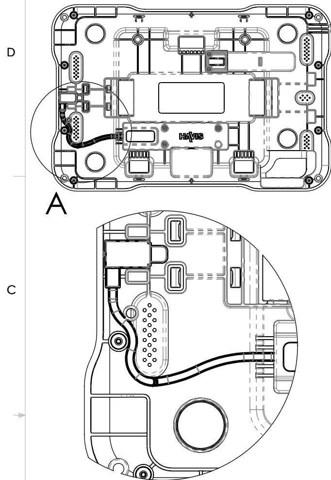
DETAIL A SCALE 2 : 3
