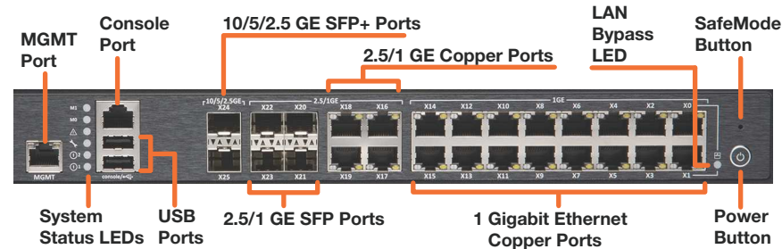
NS a 4650 Front Panel
