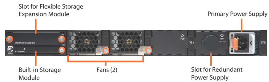
NS a 4650/5650/6650 Back Panel
