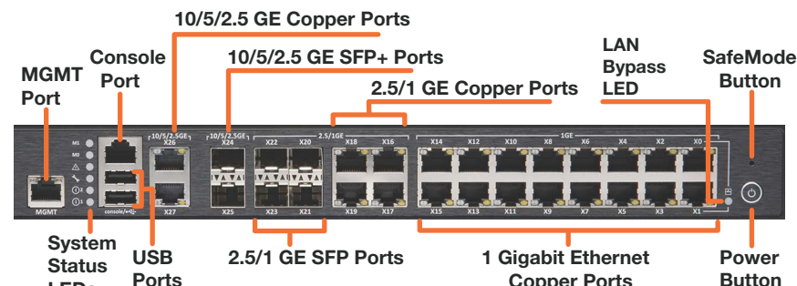
NS a 6650 Front Panel
