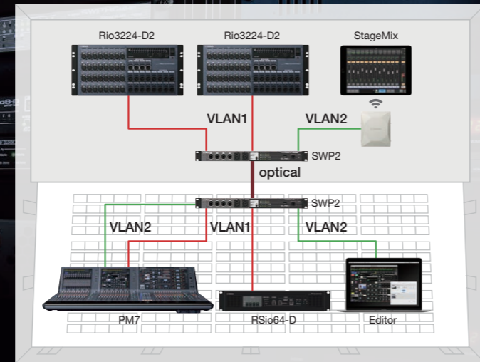
Example 2: VLAN for separating control signals from audio signals
