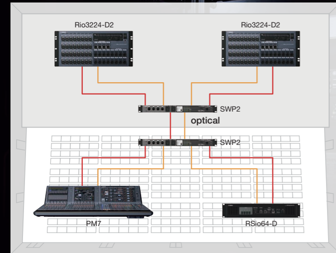
Example 1: Redundant Dante network with VLAN
