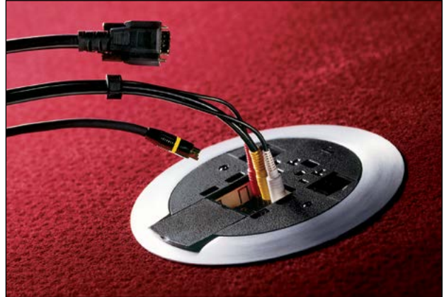
Ratchet-Pro Series Floor Box installations provide easy access to power, communication and A/V services in open spaces.
