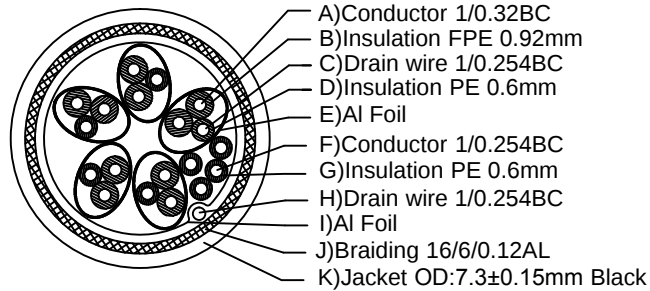
Cable Spec.
