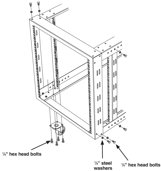
Figure 1. Assembly of the 4-Post Modular Rack.
