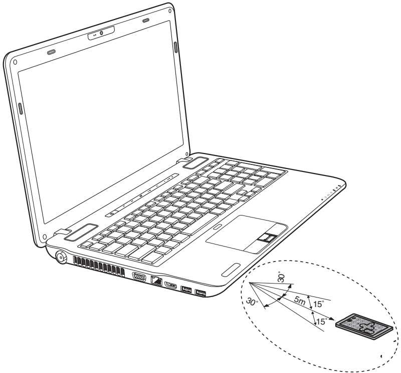
Figure 2-13 Operational range of the remote control
