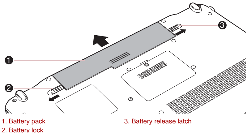
Figure 6-1 Releasing the battery pack
