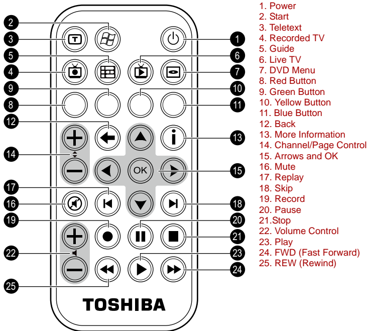
Figure 2-12 Remote Controller
