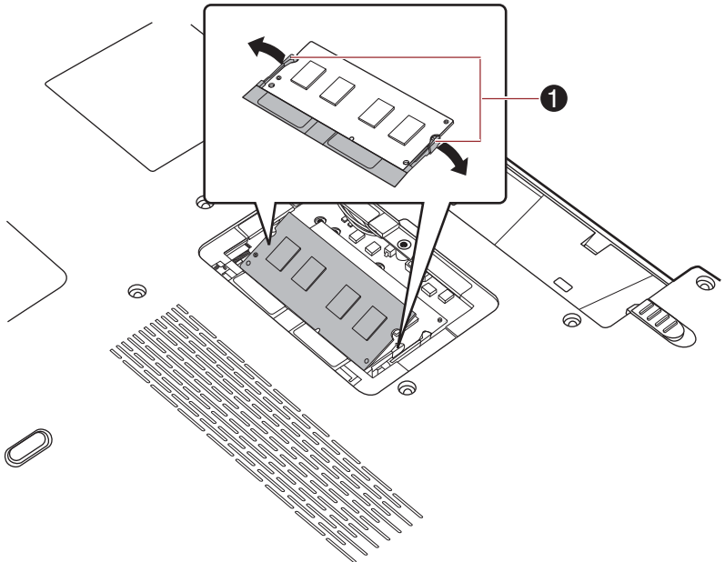
Figure 3-6 Removing the memory module
