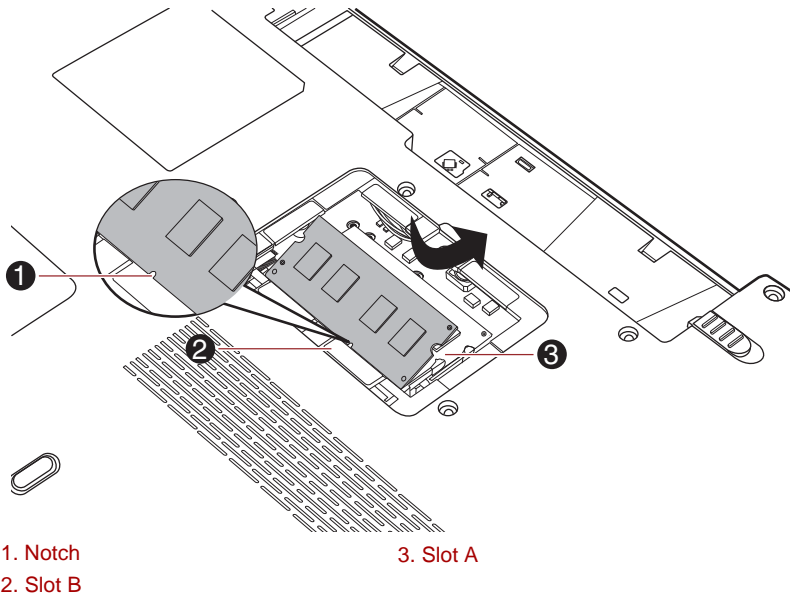
Figure 3-4 Seating the memory module
