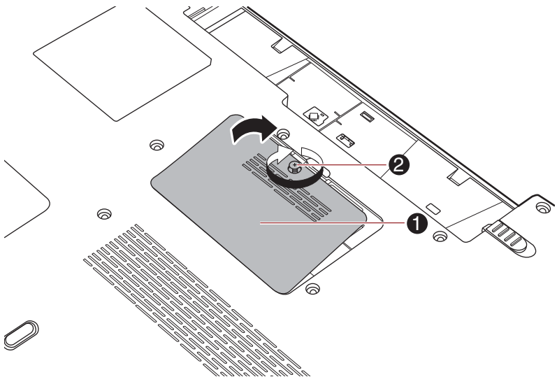
Figure 3-5 Seating the memory module cover
