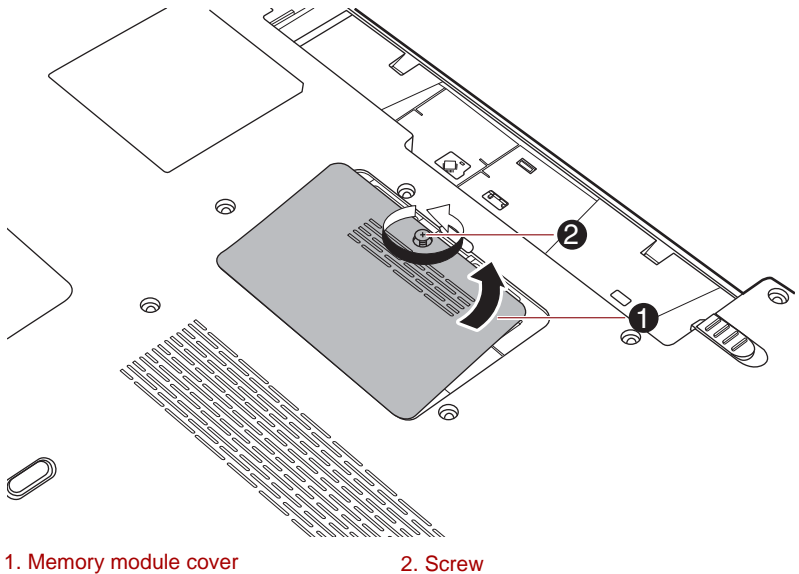
Figure 3-3 Removing the memory module cover
