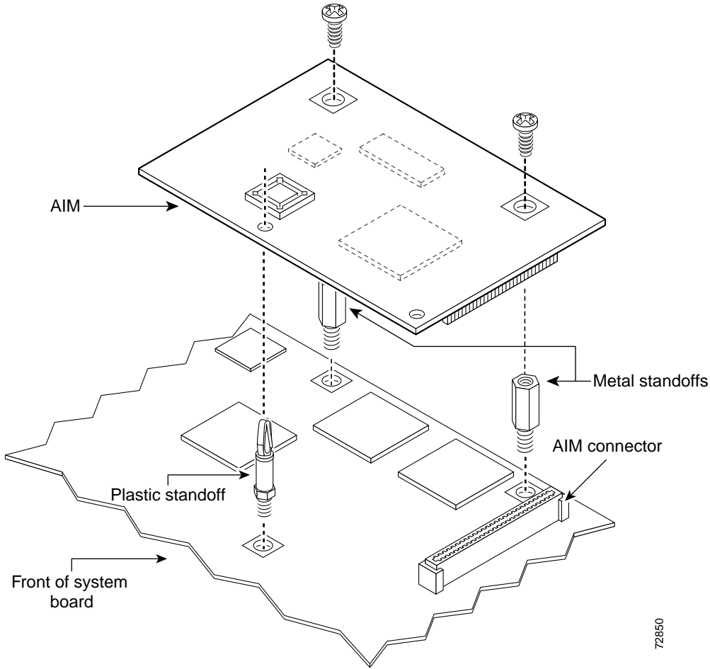
Figure 8 Connecting an AIM to the System Board
