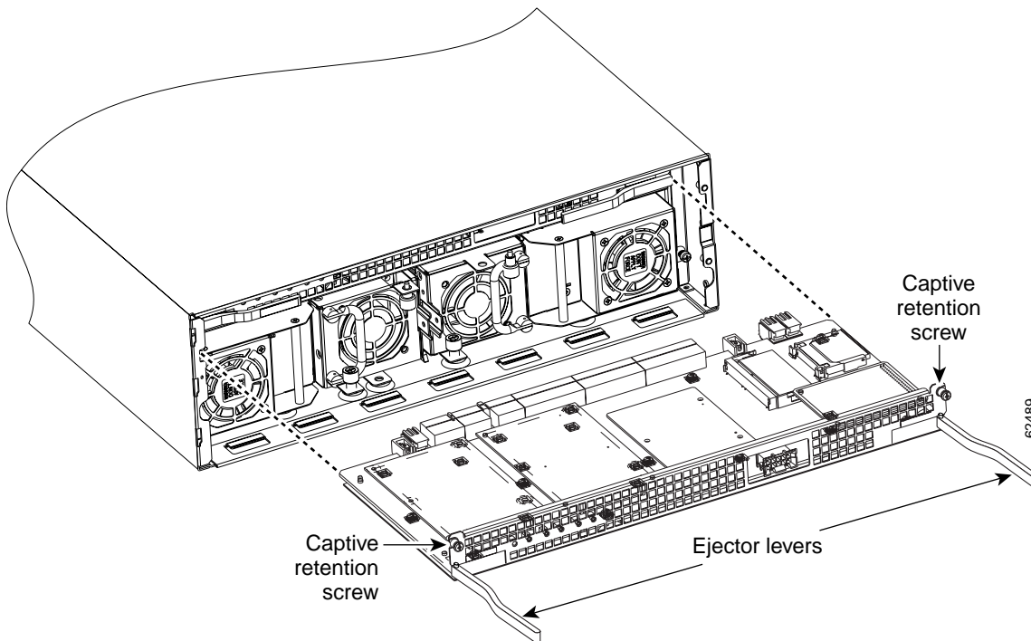
Figure 12 Reinstalling the CPU/Mainboard
