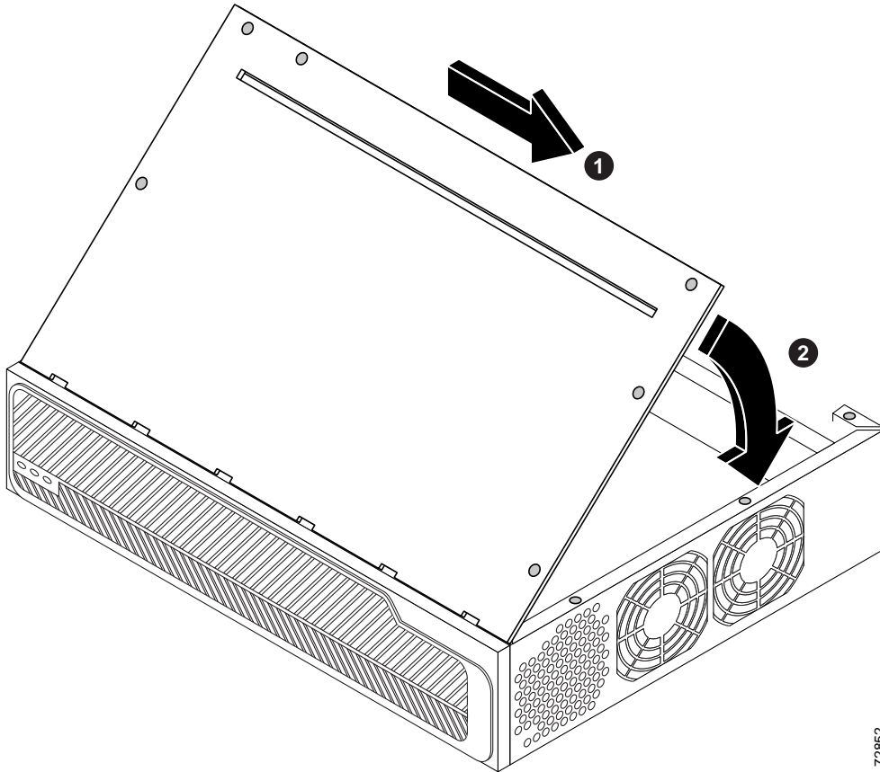
Figure 11 Replacing the Cover on a Chassis of 2-RU Height
