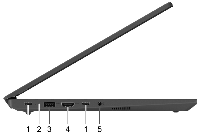
Figure 4. Lenovo V14 G6 ITN—left-side view
