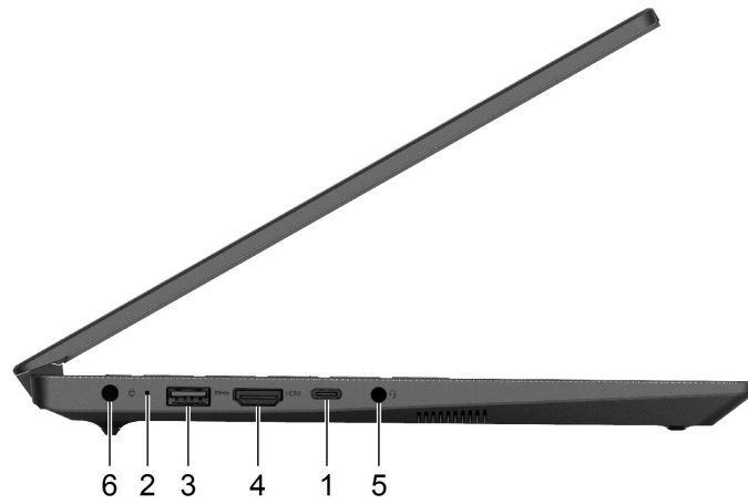
Figure 5. Lenovo V14 G6 ARP—left-side view
