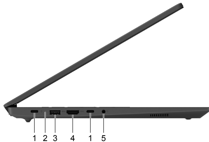
Figure 6. Lenovo V15 G6 ITN—left-side view
