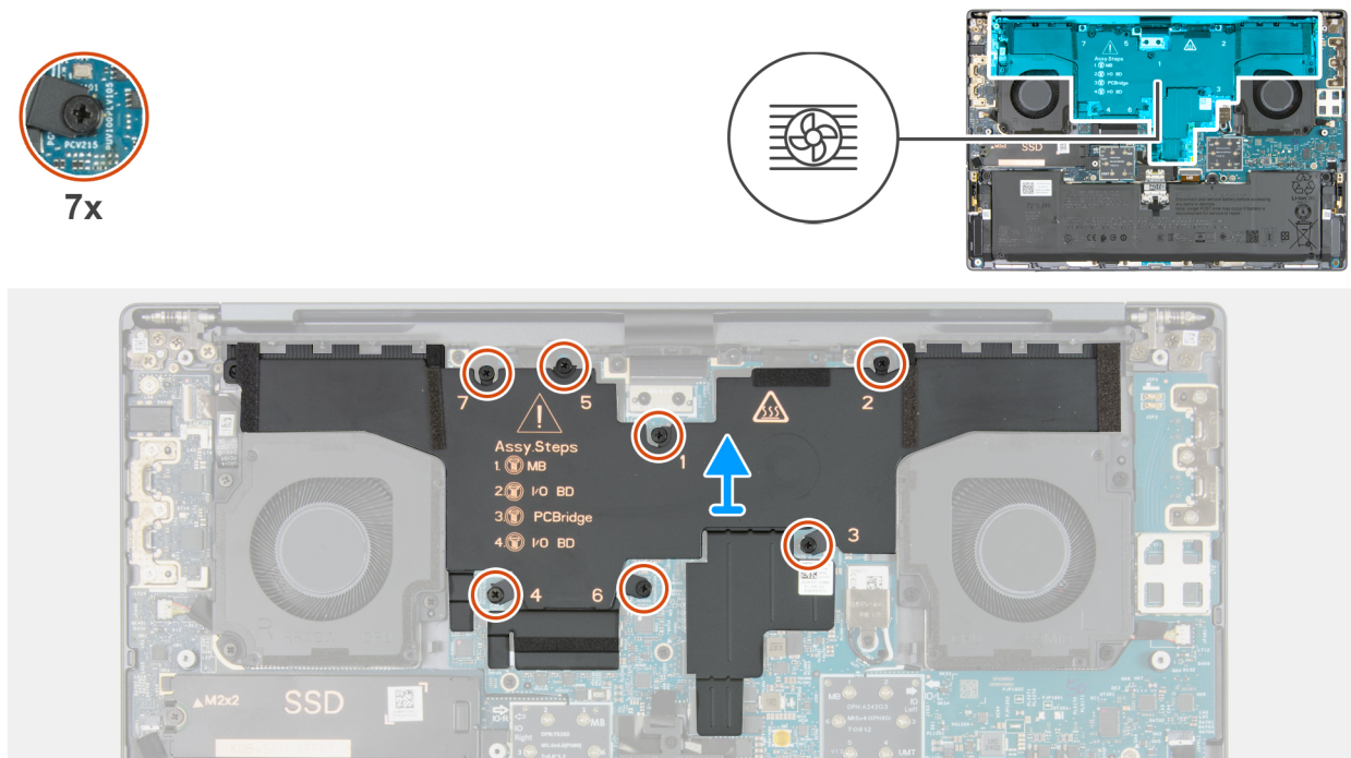
Figure 43. Removing the heat sink
