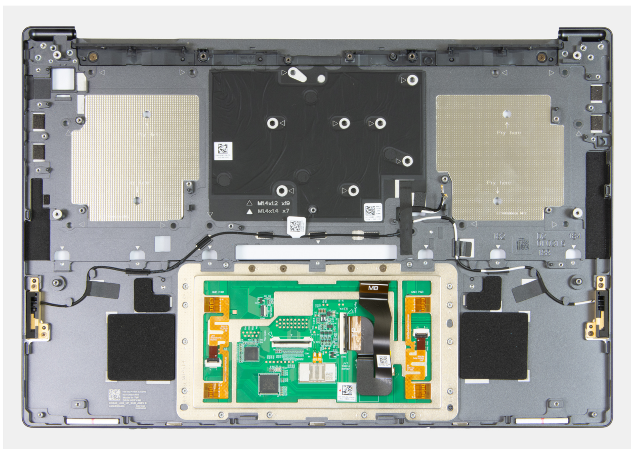
Figure 79. Palm rest and touchpad assembly
