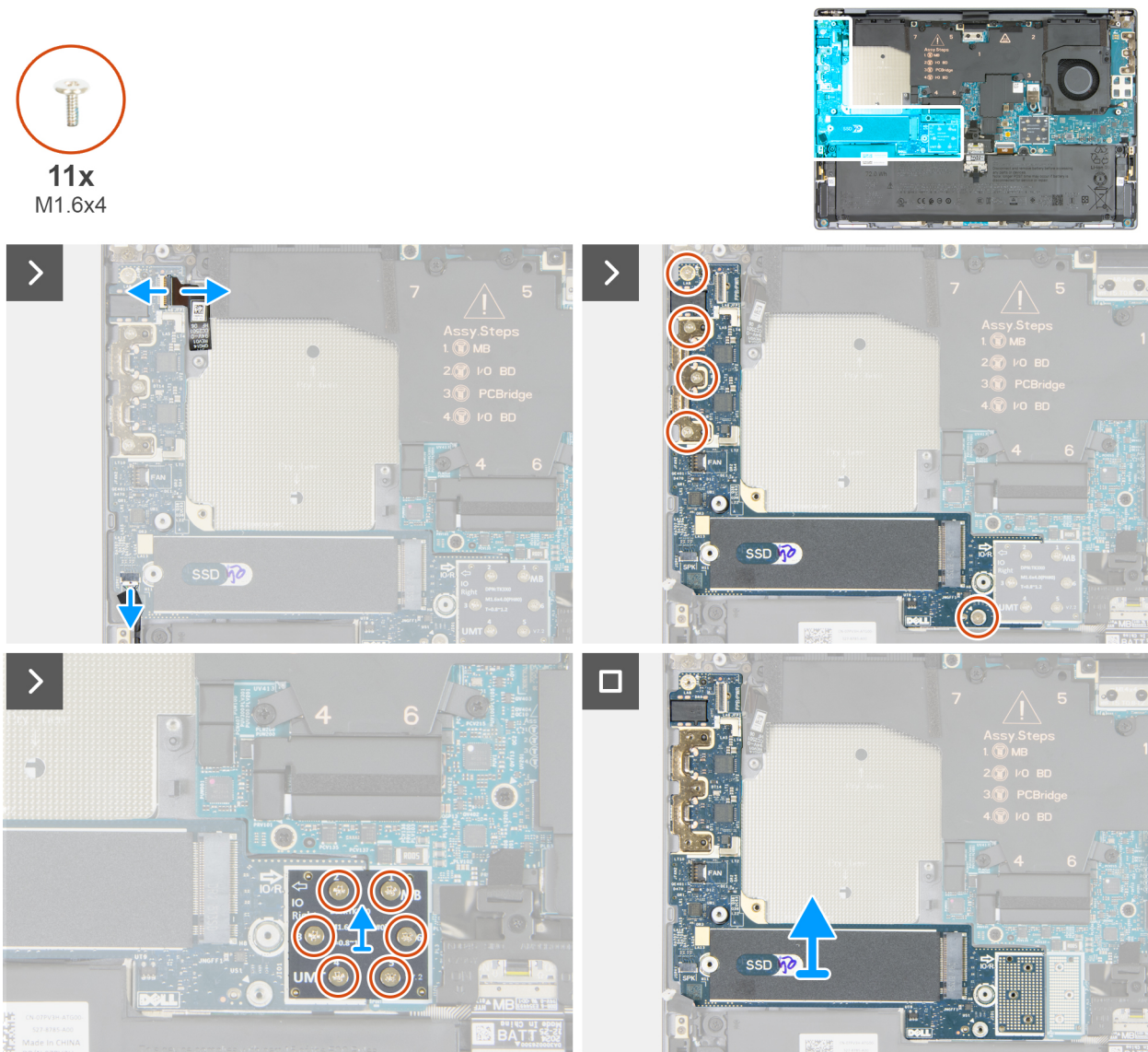
Figure 47. Removing the right I/O-board
