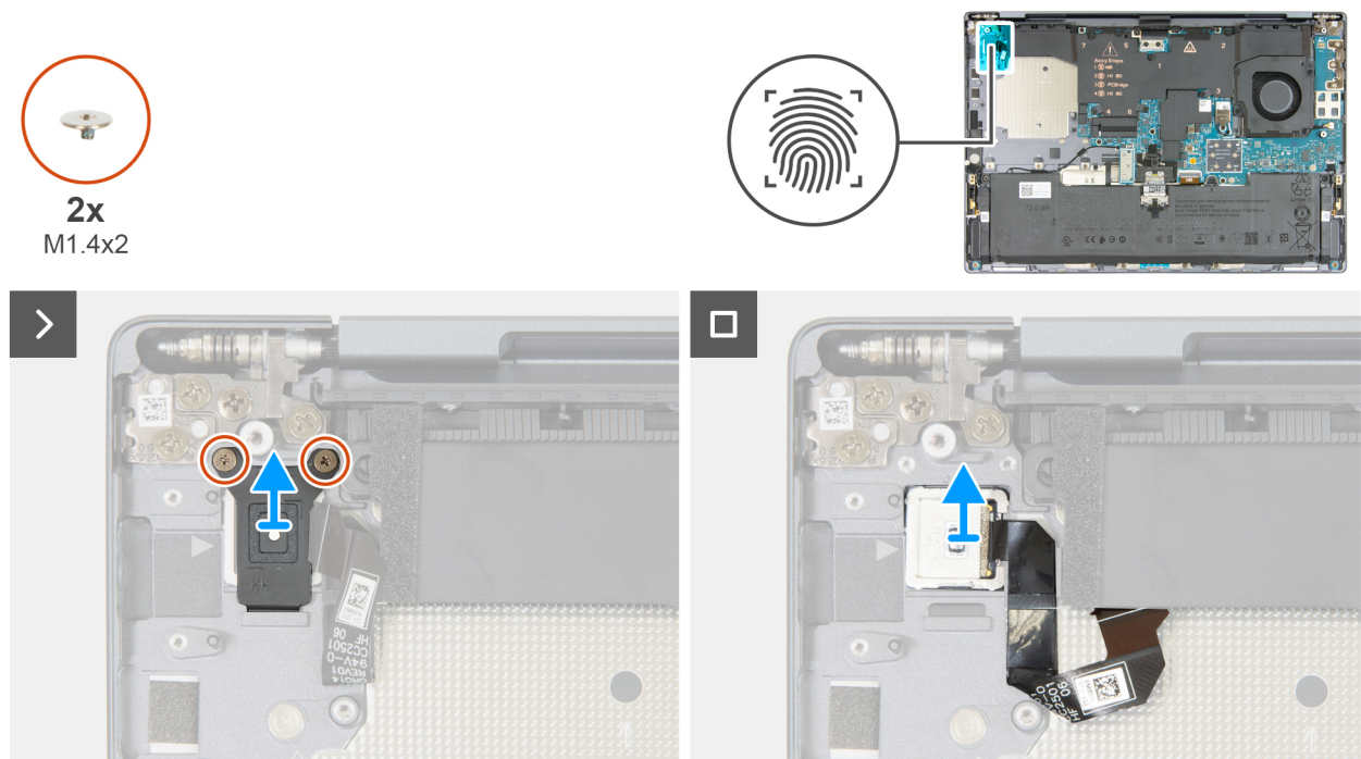
Figure 67. Removing the power button or fingerprint reader
