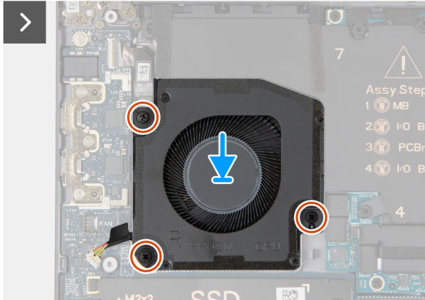
Figure 30. Installing the right fan
