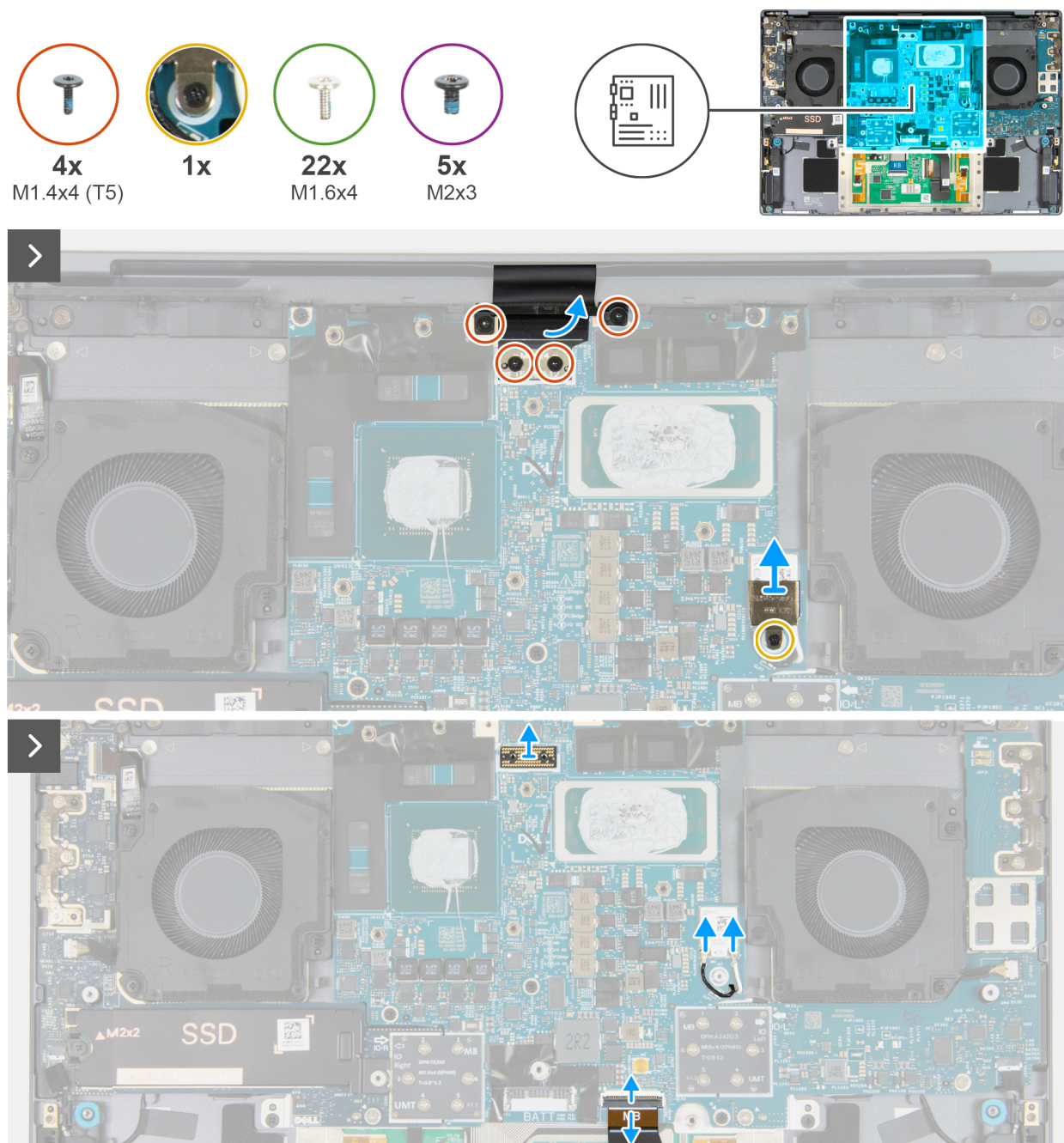
Figure 59. Removing the system board (discrete graphics)
