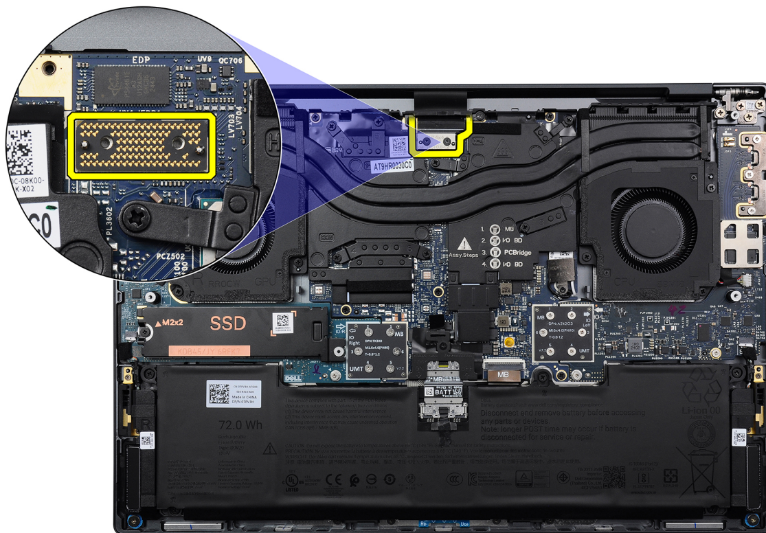
Figure 35. Display-assembly cable interposer board
