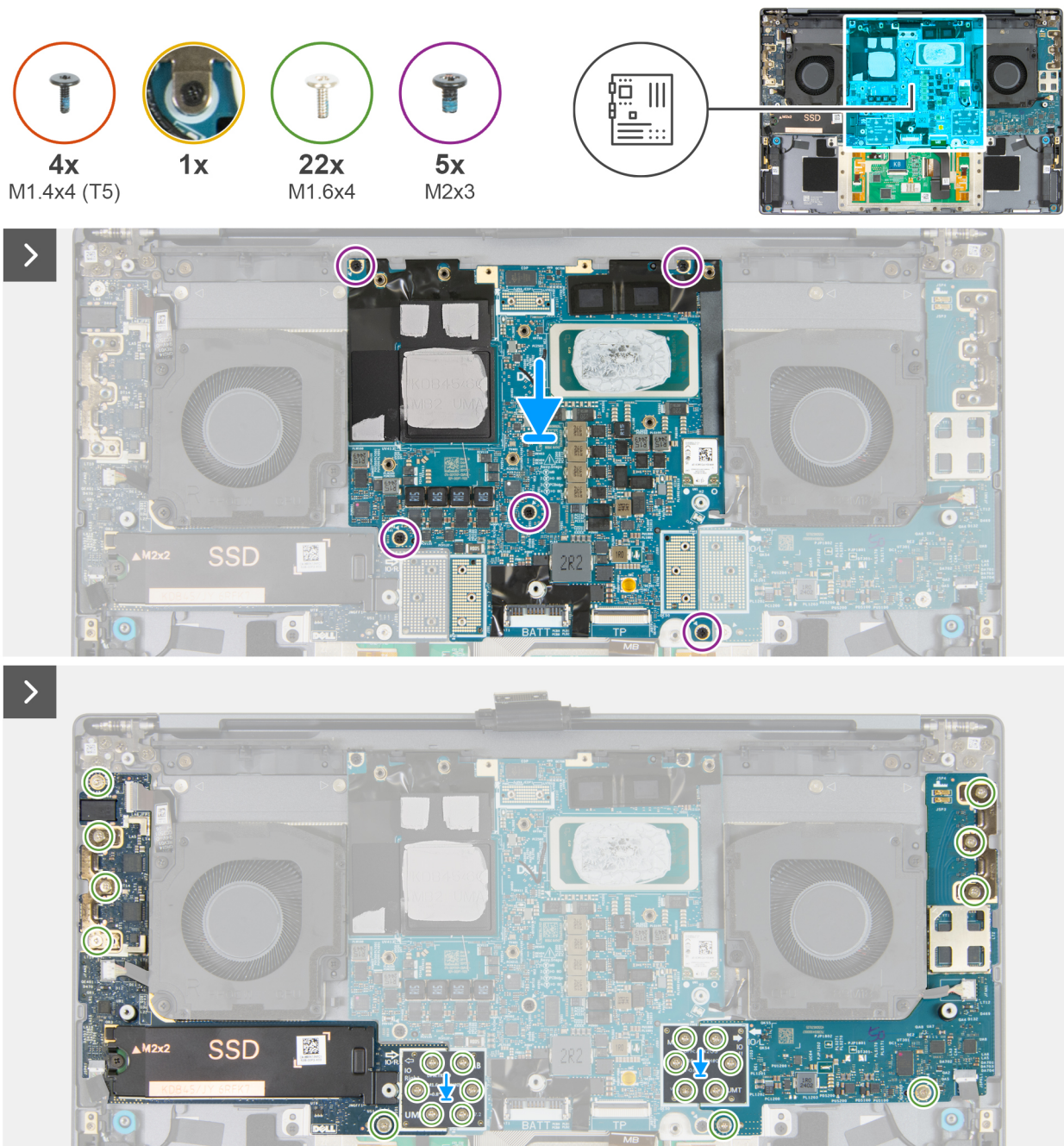
Figure 54. Installing the system board (integrated graphics)
