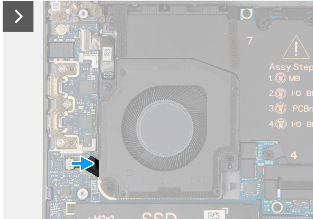
Figure 29. Removing the right fan
