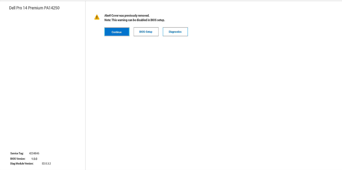
Figure 83. BIOS-Setup
