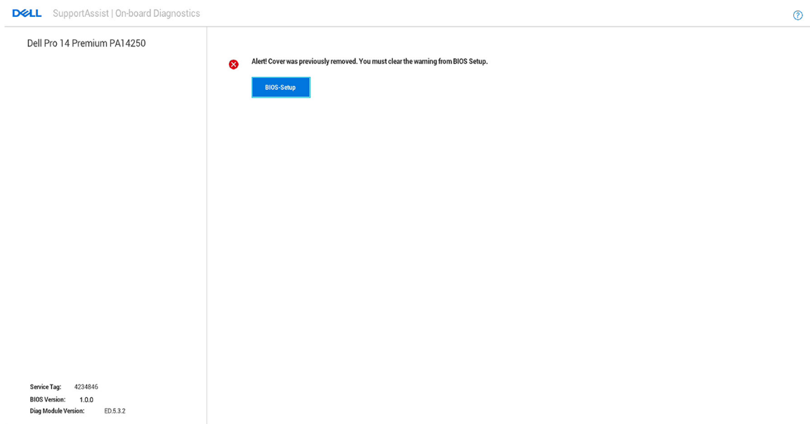
Figure 82. BIOS-Setup
