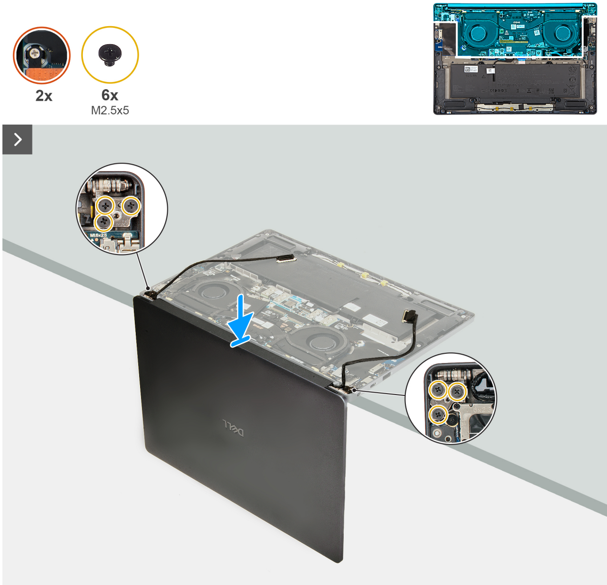
Figure 65. Installing the display assembly
