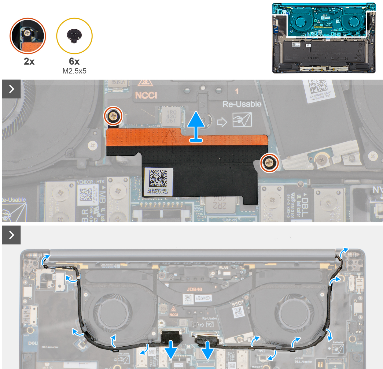
Figure 62. Disconnect the display and camera cables
