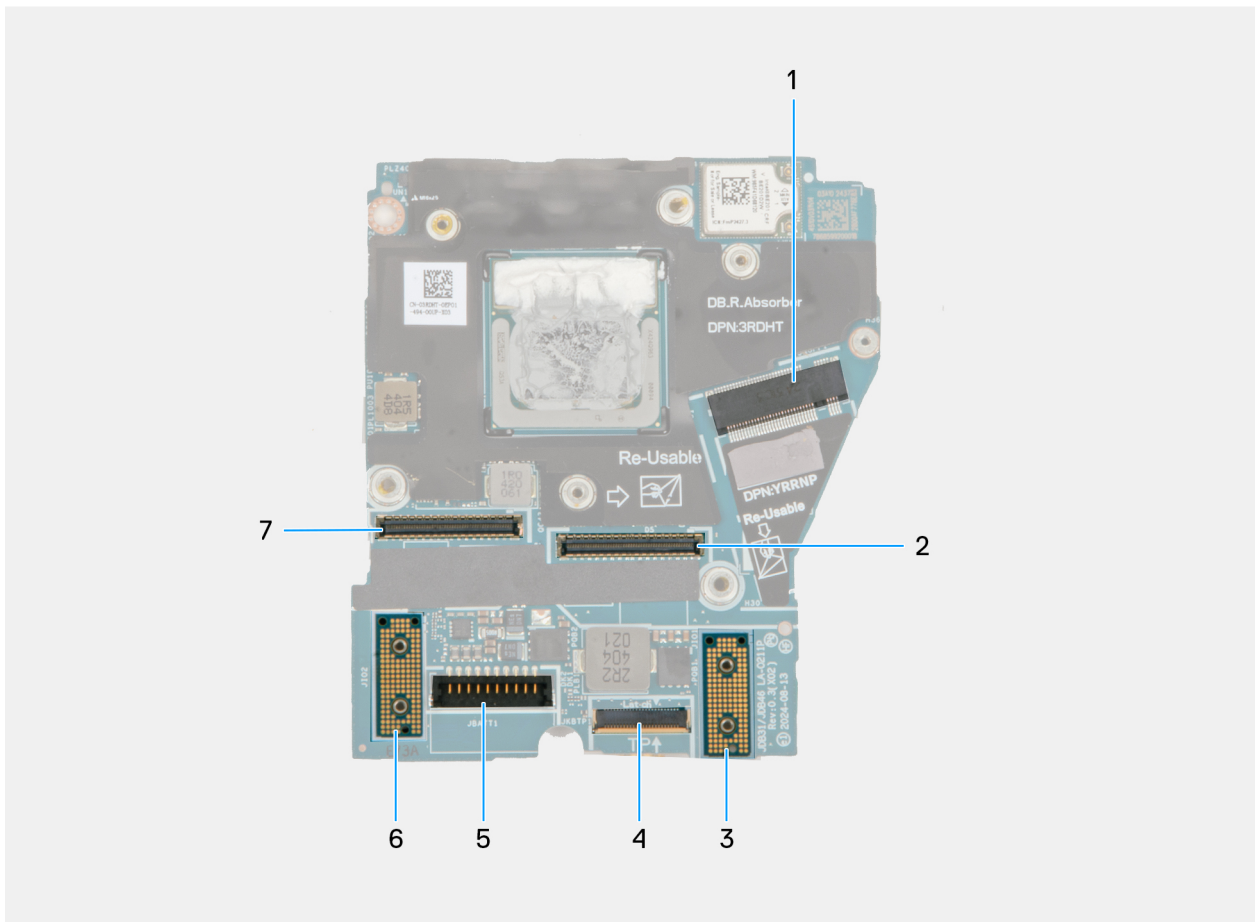
Figure 71. System board callout
