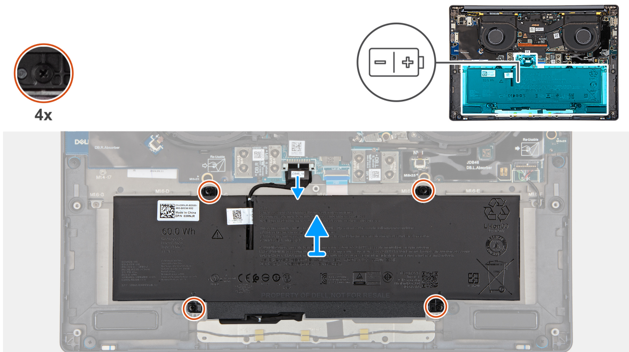
Figure 22. Loosen the captive screws
