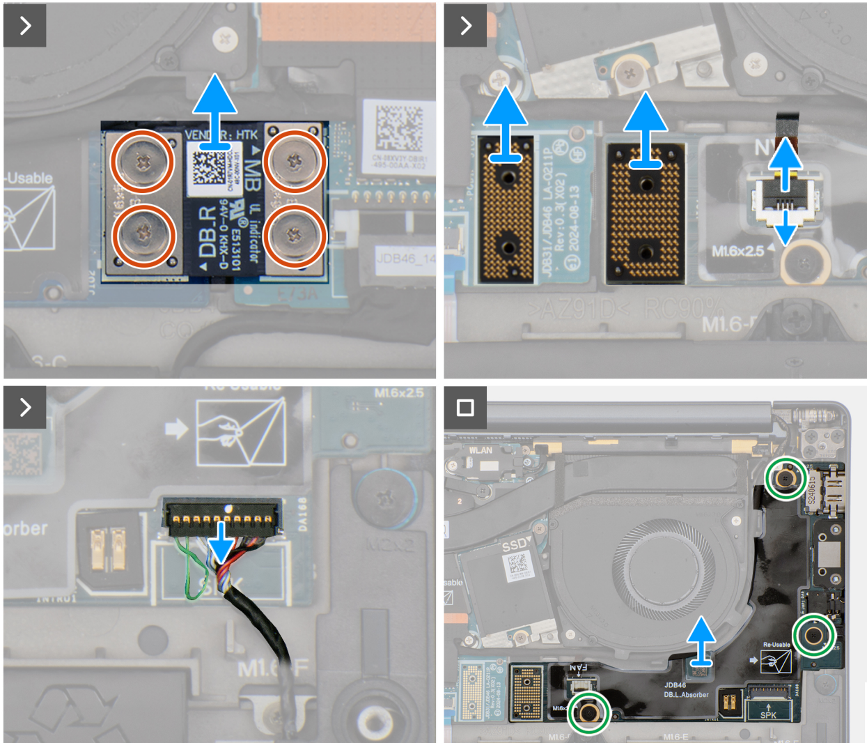
Figure 40. Removing the left I/O-board
