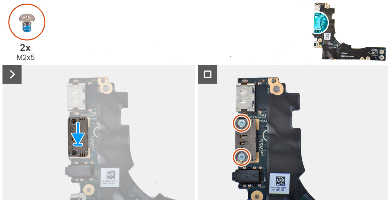
Figure 59. Installing the right USB Type-C module
