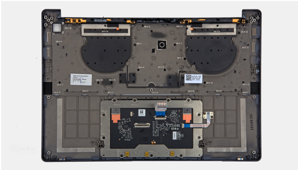
Figure 80. Palm-rest
