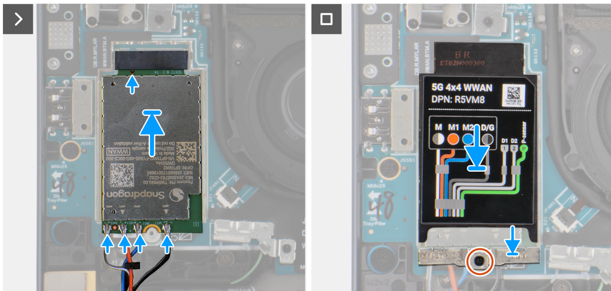
Figure 29. Installing the WWAN card
