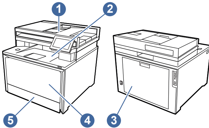
Figure 9-7 Jam locations
